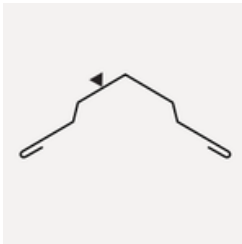
Ridge/Cottage Hip Cap FR-6
